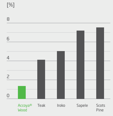
Typical tangential shrinkage from fully soaked to oven dry - the most extreme laboratory test.
